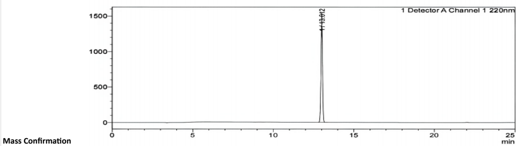
Chromatogram
